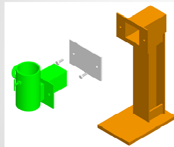
Welded to Roof Parapet Davit Support Shown w/ Portable Socket and Cover Plate
