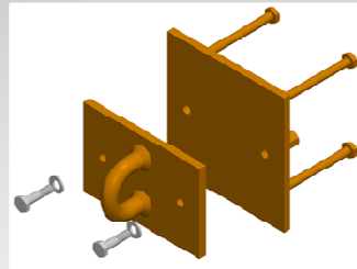
Flush Mounted Tie Back Anchor
