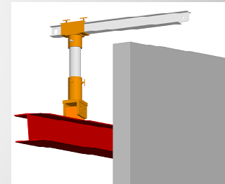
Welded Davit Base to I-Beam Shown w/ Portable Socket and Davit Assembly
