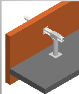
Roof Mounted Outrigger Support w/ Aluminum Boom Also Available in Parapet Mount
