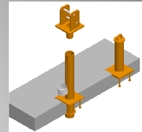
Rigging Slaves w/ Portable Rigging Socket & Cap Shown w/ Safety Tieback Anchor
