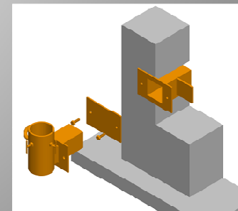
Parapet Mounted Davit Support Shown w/ Portable Socket and Cover Plate
